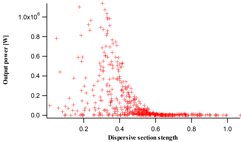
Figure 5.2: Third harmonic power as a function of the dispersive section strength (in “GENESIS” units).
