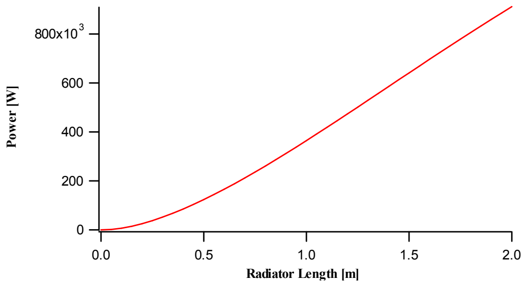
Figure 5.6: Output power along the radiator at 87 nm.
