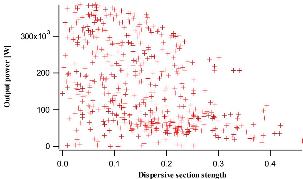
Figure 5.11: Second harmonic power as a function of the dispersive section strength (in “GENESIS” units).
