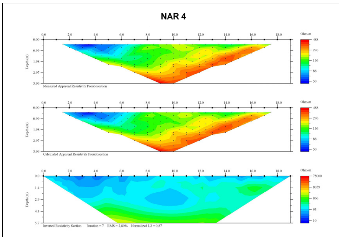
Figure 12.3: The observed apparent resistivity pseudosections for the Nariče (NAR 4) together with inversion models.
