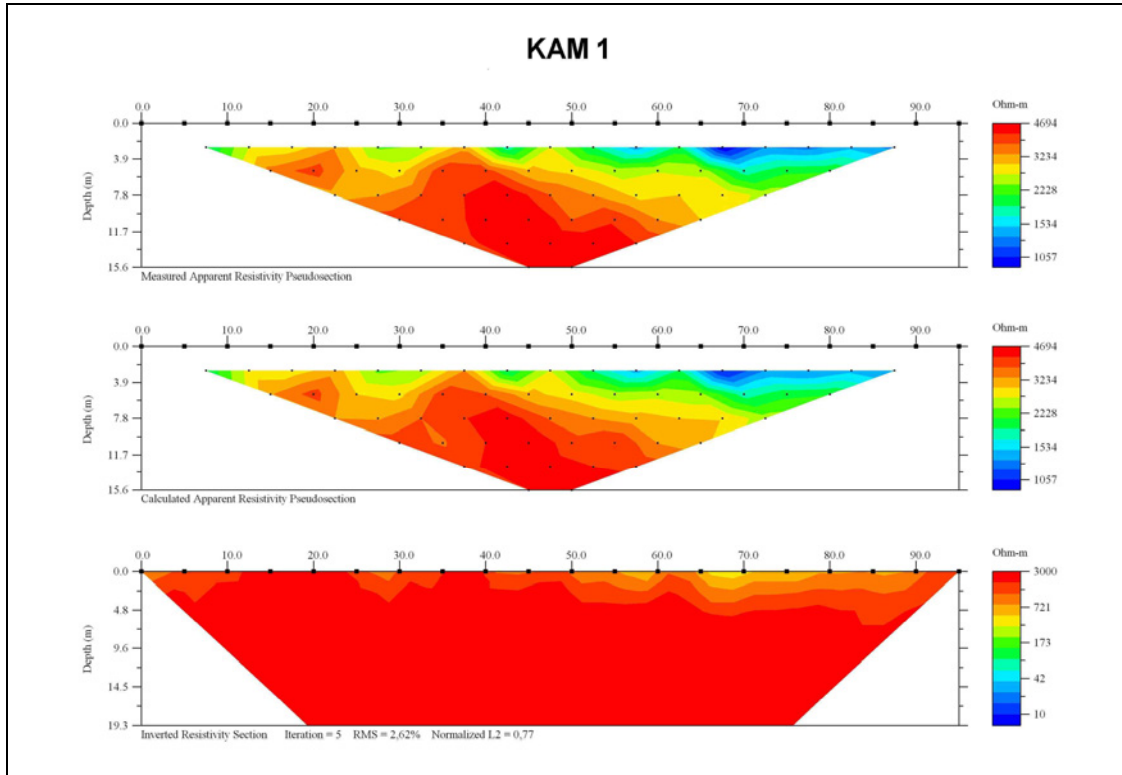
Figure 9.38: The observed apparent resistivity pseudosections for the Kamenščina dry valley (KAM 1) together with inversion models.
