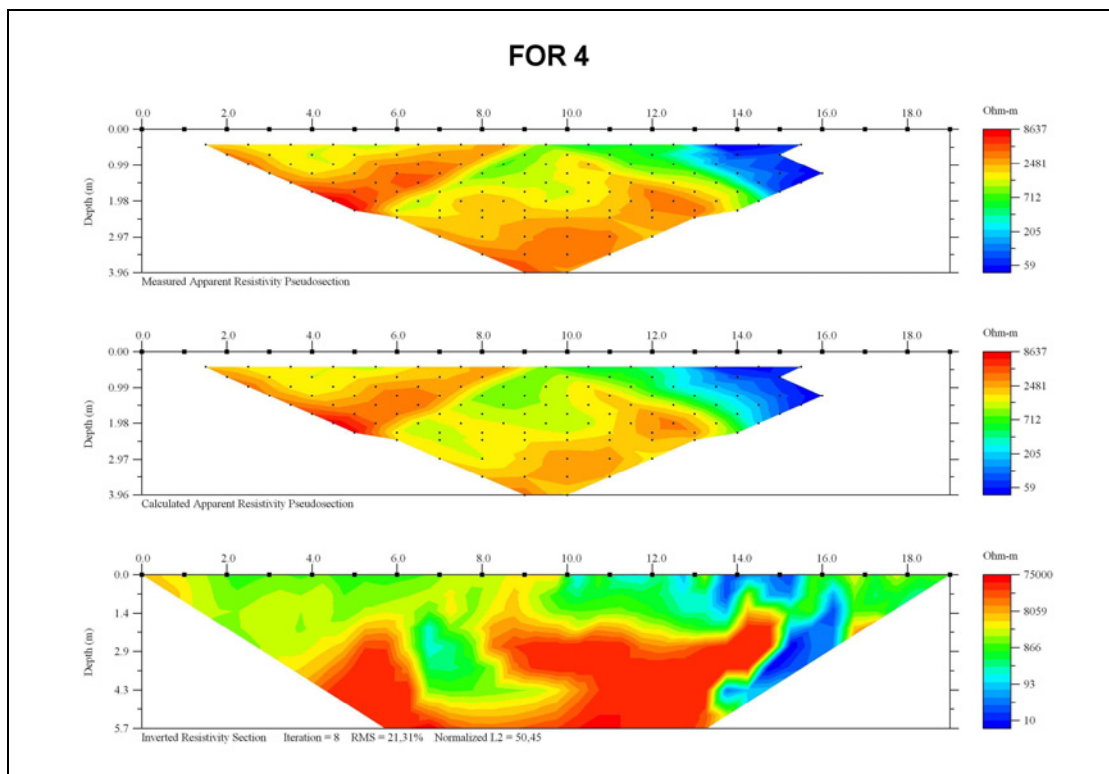
Figure 12.5: The observed apparent resistivity pseudosections for the area northeast of the Šembije village (FOR 4) together with inversion models.
