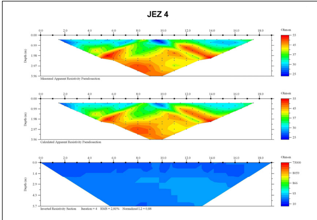
Figure 12.2: The observed apparent resistivity pseudosections for the Šembijško Jezero (JEZ 4) together with inversion models.
