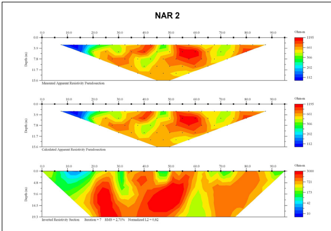
Figure 9.37: The observed apparent resistivity pseudosections for the Nariče (NAR 2) together with inversion models.
