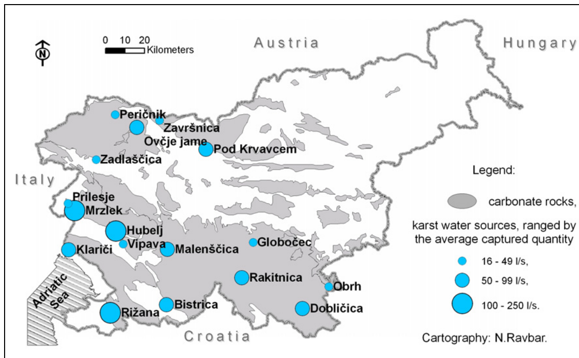
Figure 3.1: Schematic map showing the extent of carbonate rocks outcrops and some of the most important karst water sources.
