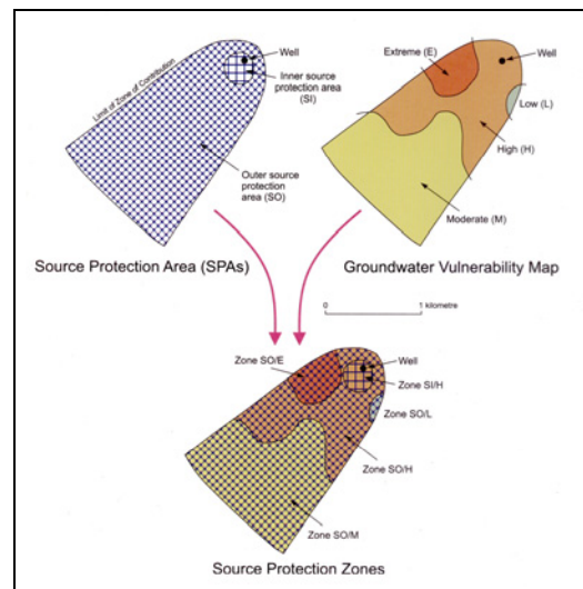
Figure 5.4: Illustration of the source protection zones delineation from the Irish method by the integration of the source protection area map and the vulnerability map (Groundwater Protection Schemes, 1999).
