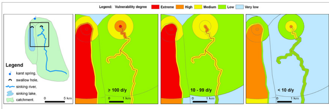
Figure 7.6: Integrating temporal variability tv sub-factor into the existing C score assessment scheme by adding it to the product of dh , ds and sv sub-factors.
