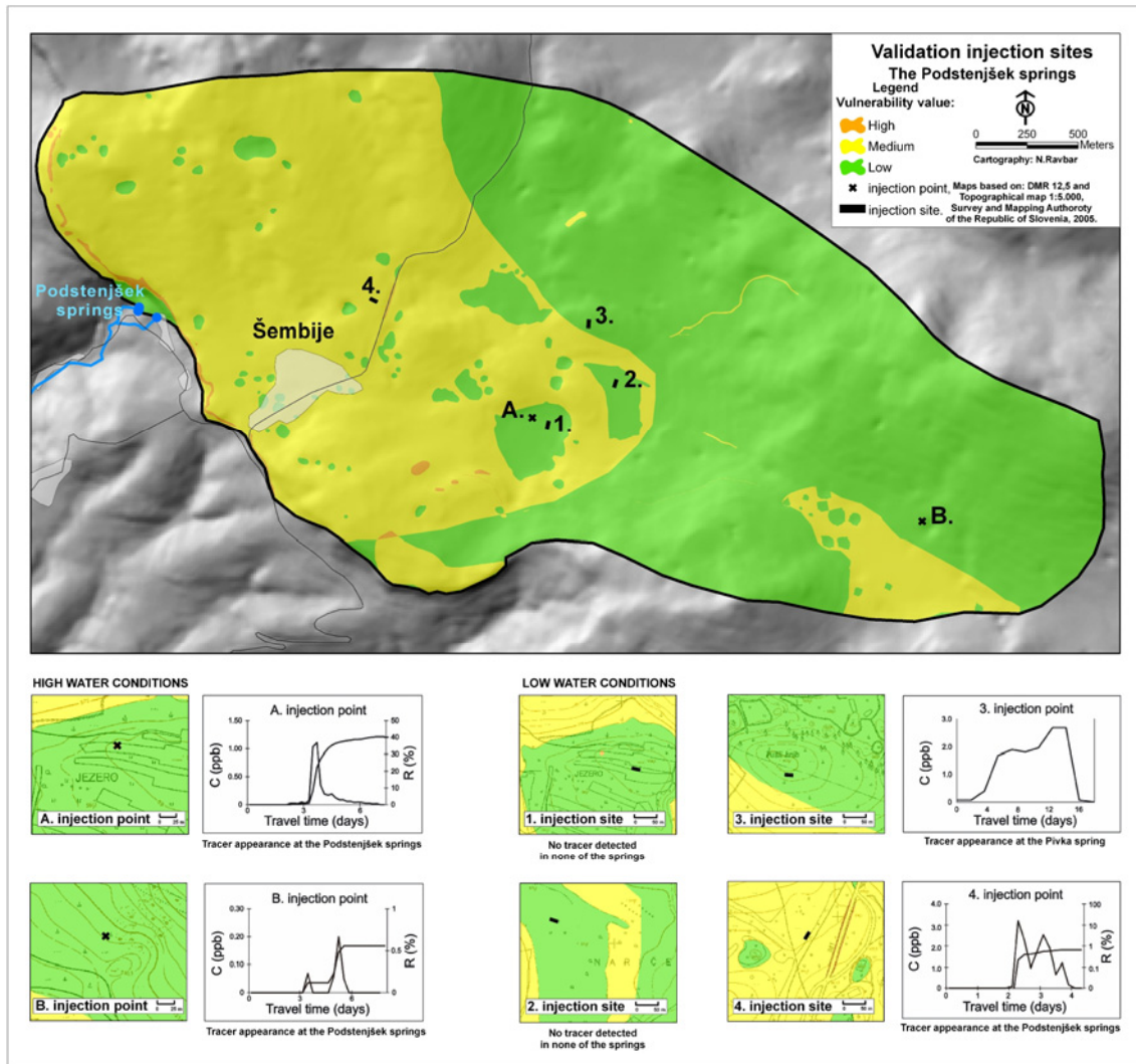
Figure 12.12: Slovene Approach source vulnerability of the test site detailed scale insets of the validation points under different hydrological conditions and obtained results.
