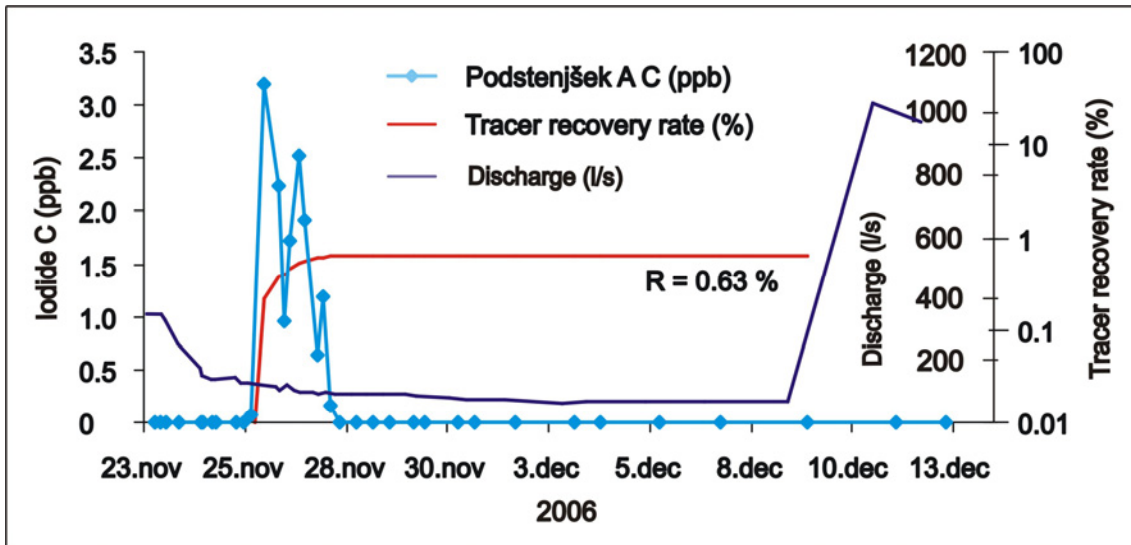
Figure 12.10: Iodide breakthrough curve observed in the Podstenjšek spring.
