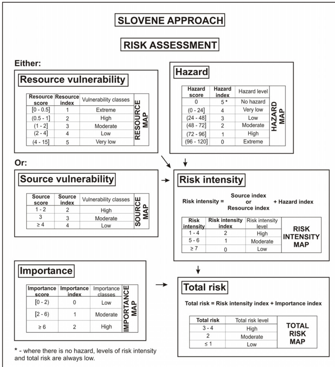
Figure 8.5: Slovene Approach to total risk assessment.
