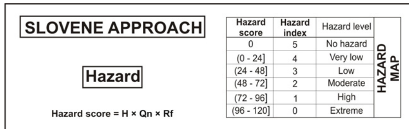
Figure 8.3: Hazard assessment scheme.
