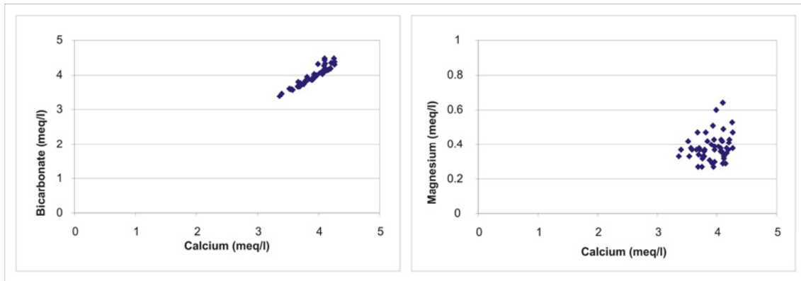
Figure 9.17: Calcium, bicarbonate and magnesium concentrations of the Podstenjšek springs (source: Kogovšek, 2006).
