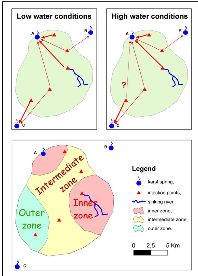
Figure 7.11: Illustration of the A source catchment division into inner, intermediate and outer zone.
