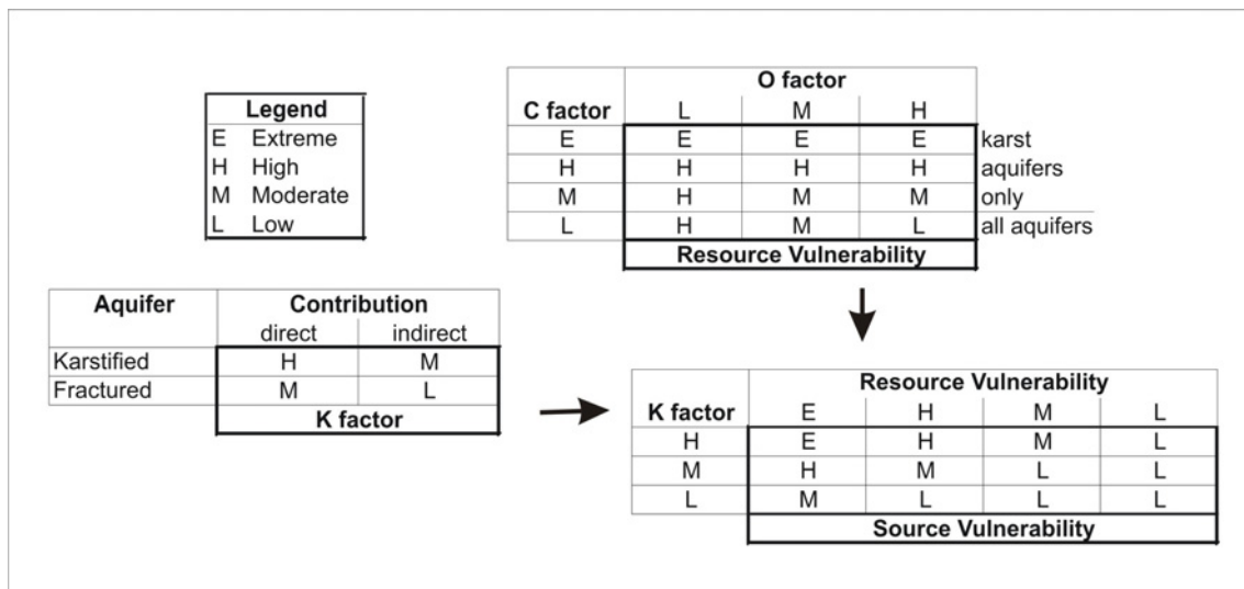
Figure 5.9: Assessment scheme for source vulnerability mapping proposed in addition to the Simplified method.
