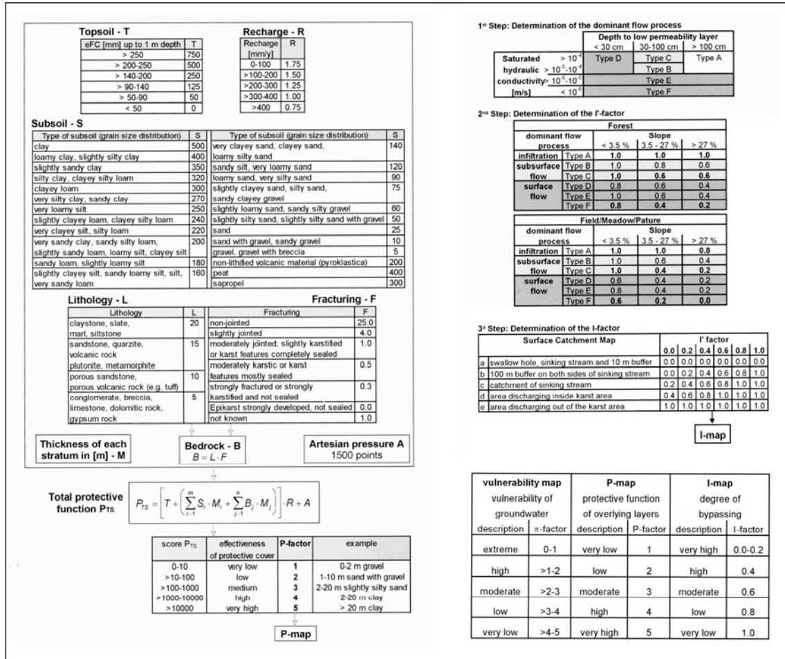
Figure 5.3: Assessment of the P and I parameters, as well as the PI vulnerability map assessment (Goldscheider, 2002).
