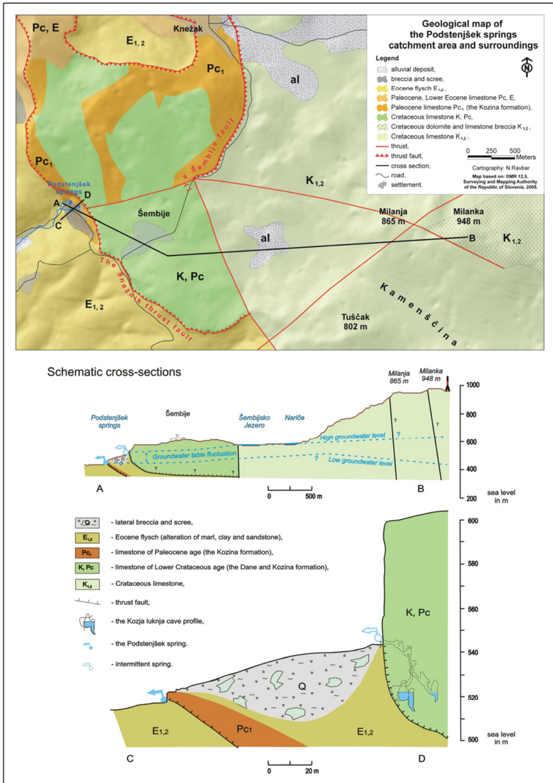
Figure 9.3: Geological map of the Podstenjšek springs catchment area and surroundings and schematic cross-sections of the hydrogeological characteristics of the area (after Šikić et al., 1972; Šikić and Pleničar, 1975; Buser, 1976; Placer, 1981; Krivic et al., 1983; Poljak, 2000).
