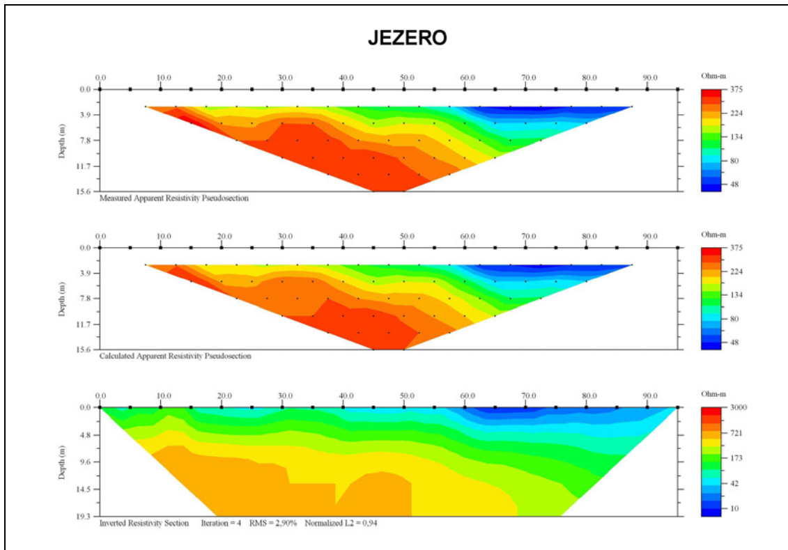
Figure 9.35: The observed apparent resistivity pseudosections for the Šembijško Jezero (JEZERO) together with inversion models.
