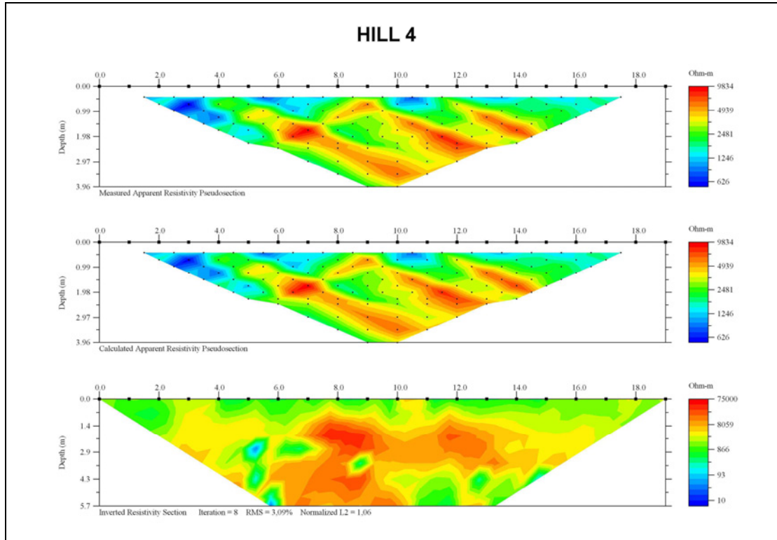
Figure 12.4: The observed apparent resistivity pseudosections for the Pušli hrib (HILL 4) together with inversion models.
