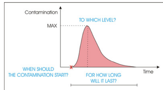
Figure 5.1: The three basic questions that have been initiated into the groundwater vulnerability mapping concept (Brouyère, 2004).
