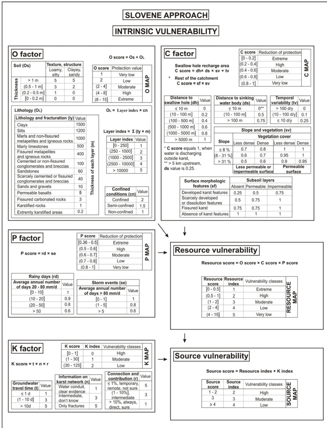
Fig. 7.12: Slovene Approach to resource and source intrinsic vulnerability assessment scheme.
