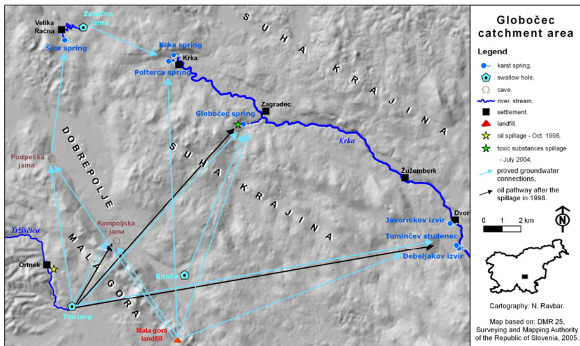
Figure 2.8: Sketch of the proved groundwater connections in the Globočec catchment area and places of the contamination events (after Novak, 1987; Kogovšek and Petrič, 2002; Kogovšek et al. , 2005).
