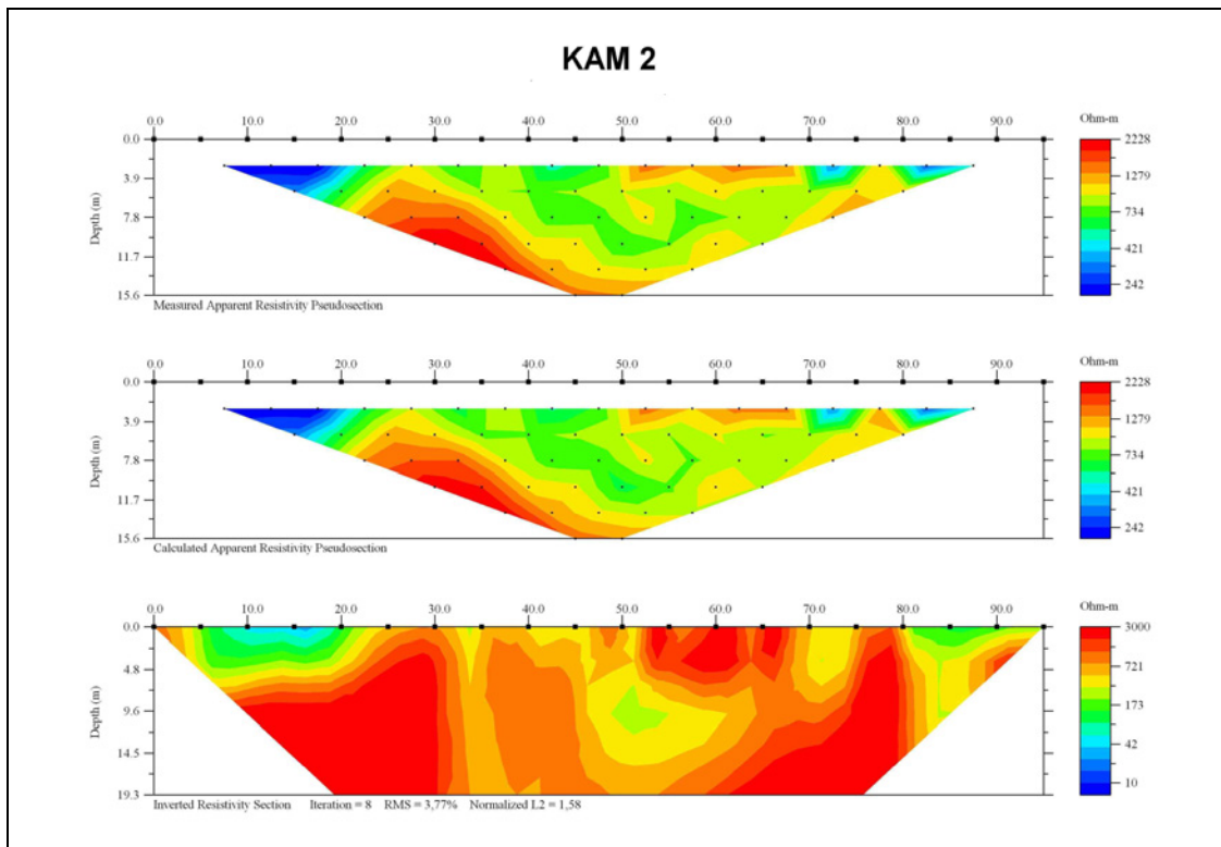
Figure 9.39: The observed apparent resistivity pseudosections for the Kamenščina dry valley (KAM 2) together with inversion models.
