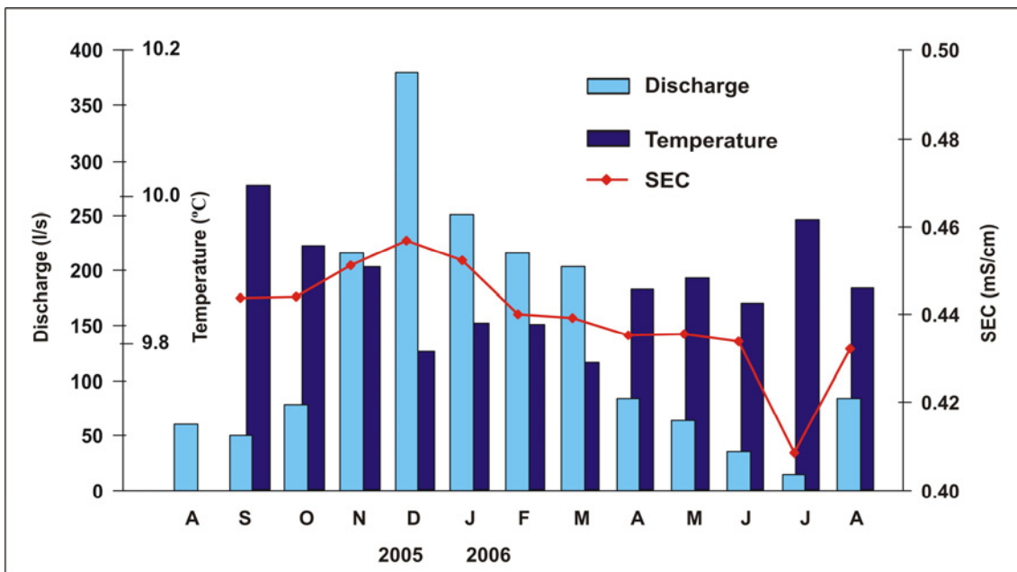
Figure 9.7: Average monthly discharges, temperature and specific electrical conductivity values of the Podstenjšek springs.
