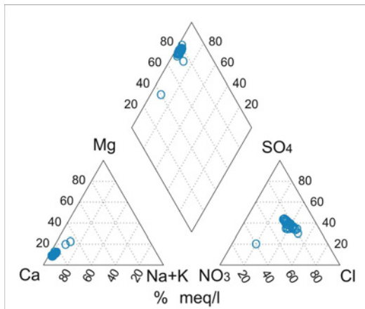
Figure 9.15: The PIPER diagram of the Podstenjšek springs.
