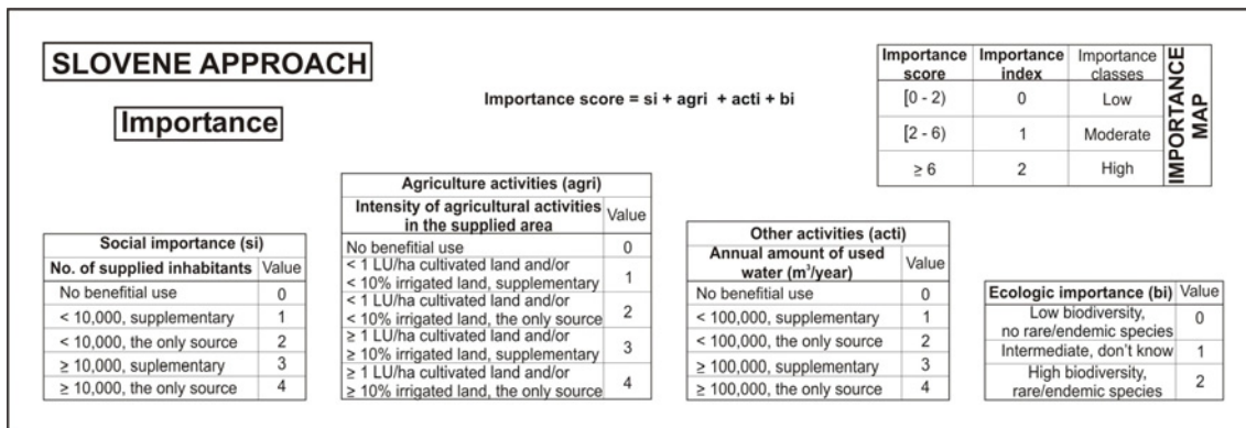
Figure 8.4: Slovene Approach to water resource/source importance assessment scheme.
