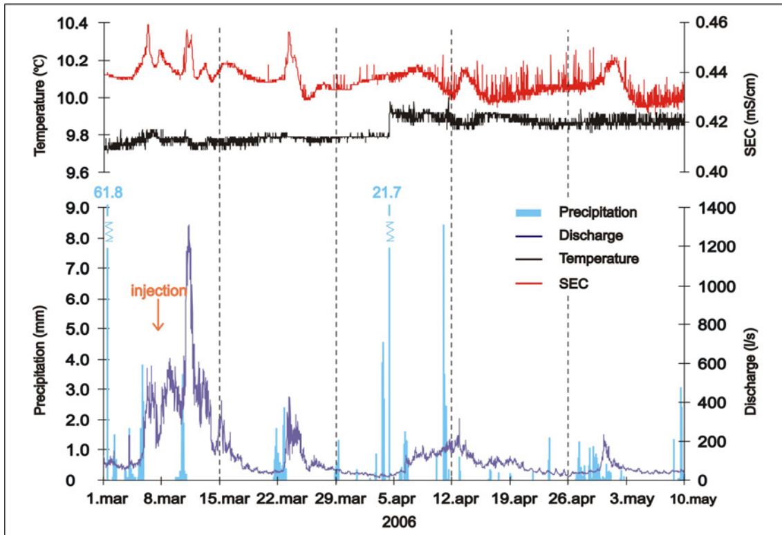
Figure 9.21: Hydrological conditions of the Podstenjšek springs in the time of the tracing test. Half hour values are displayed on the graph. Precipitation data was gained from the Slovene Environmental Agency (MOP ARSO, 2007).
