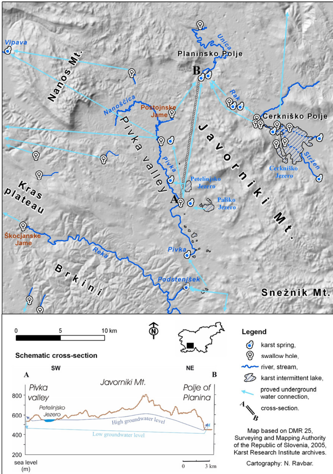
Figure 2.5: Hydrological map of the western Dinaric karst in Slovenia with some underground connections proved by tracer tests, and schematic section of the area during low- and high-water conditions with special emphasis on the Javorniki mountains, Cerknjško and Planinsko Polje and Pivka valley.
