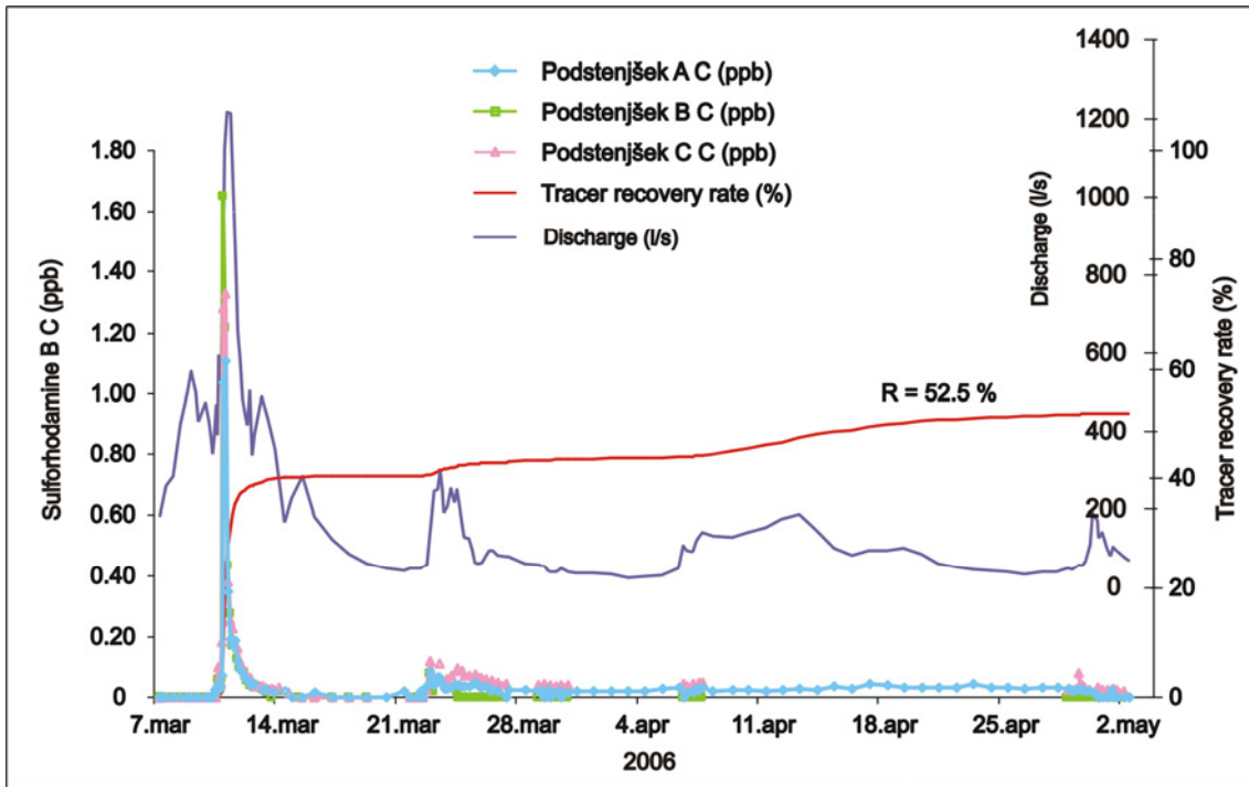
Figure 9.23: Sulforhodamine B breakthrough curve observed in the Podstenjšek springs.
